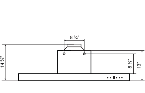
FRONT WITHOUT FLUE
