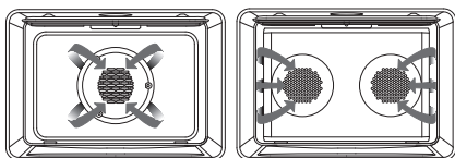
Thermal Cavity
