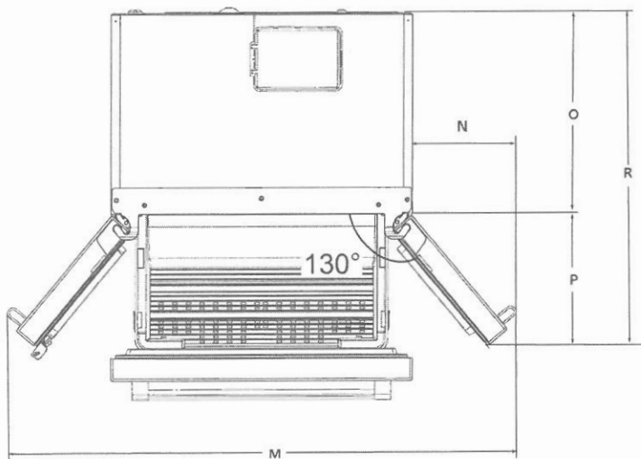
Fresh Food Door Open 130° (Max)
