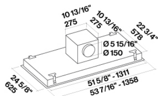
Hood with motor
